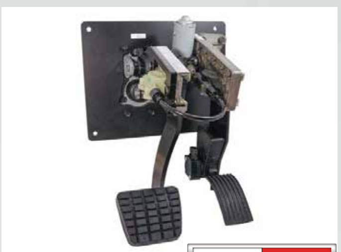
SUSPENDED PEDALS OFFERS A BETTER VIEW OF THE GAUGES, CONVENIENT ACCESS TO CONTROLS AND A MORE AUTOMOTIVE LOOK
