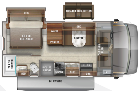
22J Ext. Lgth: 24' 8" Wheelbase: 223" GVWR: 14,500 lbs.
