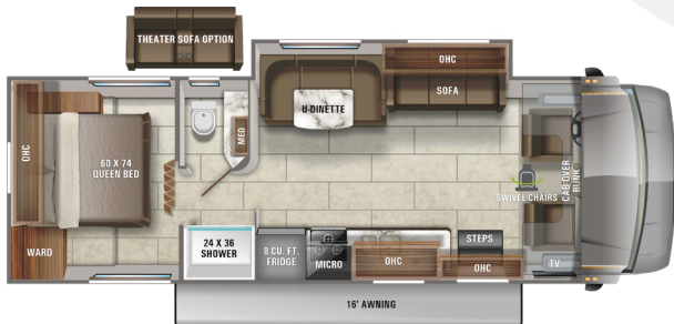
29XK Ext. Lgth: 32' 6" Wheelbase: 223" GVWR: 14,500 lbs.
