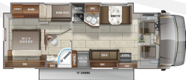
31F Ext. Lgth: 32' 6" Wheelbase: 223" GVWR: 14,500 lbs.
