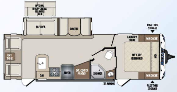
269RLSWE | Rear living, super-slide Weight: 5662 LBS. | Length: 32' 5"
