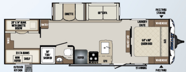
287QBSWE | Quad bunkhouse, super-slide Weight: 6002 LBS. | Length: 33' 10"
