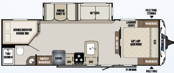
273BHSWE | Bunkhouse, super-slide Weight: 5464 | Length: 31' 3"
